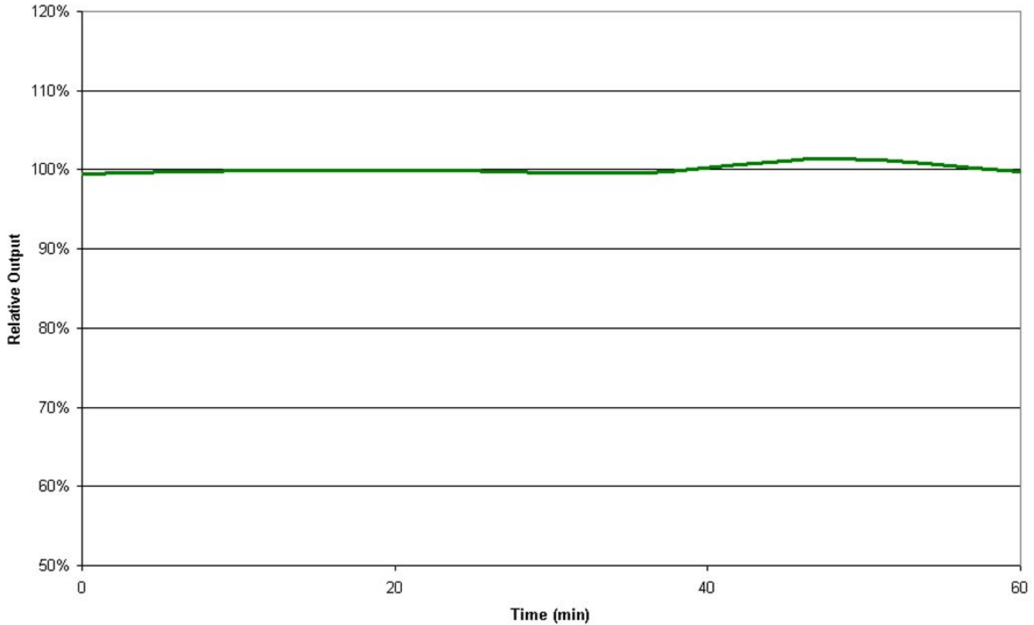
Typical Relative Stability of X-Cite 120XL over 1 Hour Period
