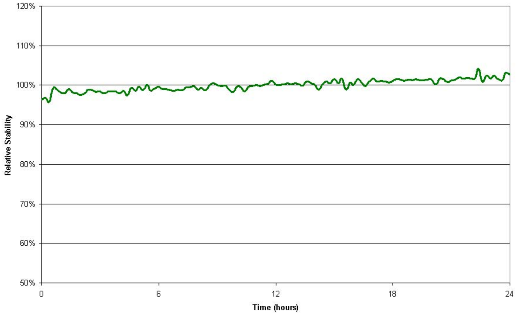
Typical 24hr Stability of X-Cite 120XL
